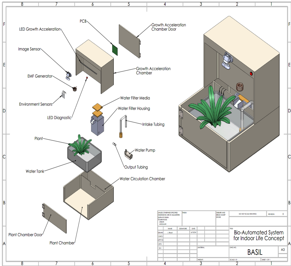
Figure 2.7 Prototype
