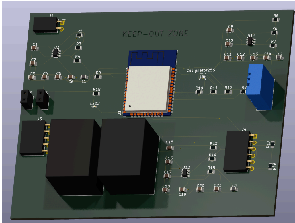
Figure 8.1 PCB Layout
