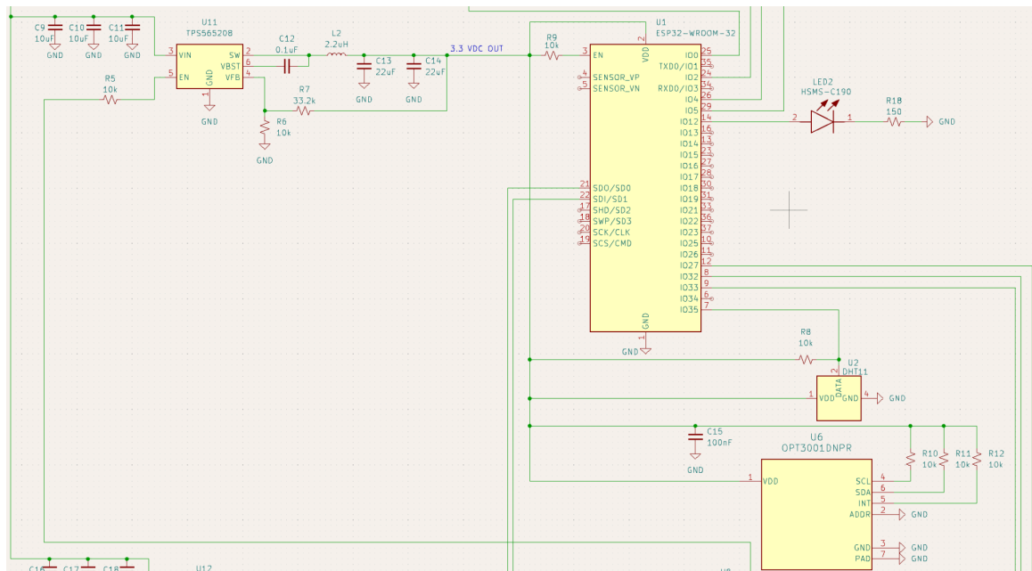
Figure 6.6. 3.3VDC Subsystem
